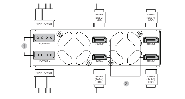
1 Molex 4 Pin Power 2 7 Pin SATA
