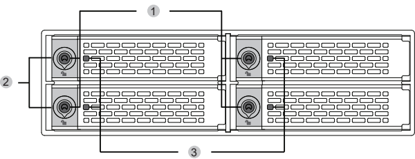
1 EZ-LOCK 2 Drive Tray Ejection Button 3 LED Indicator(Device Power : Solid Green ; Drive Access : Flashing Amber)
